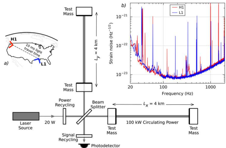
Figure 2. Simplified diagram of an Advanced LIGO detector (not to scale), including several of the key enhancements to the basic design: an optical cavity that reflects the laser light back and forth many times in each arm, multiplying the effect of the gravitational wave on the phase of the laser light; a power recycling mirror that increases the power of the laser in the interferometer as a whole; a signal recycling mirror that further optimizes the signal extracted at the photodetector . These enhancements boost the power of the laser in the optical cavity by a factor of 5000, and increase the total amount of time that the signal spends circulating in the interferometer.
